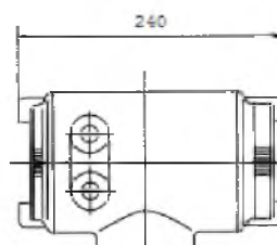
e Outline Dimension of medium and high pressure sensor M A G Y N Intelligence Transmitter (Round Type)
