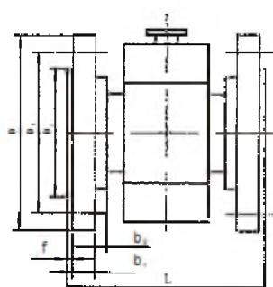
e Outline Dimension of medium and high pressure sensor M A G Y N Intelligence Transmitter (Round Type)
