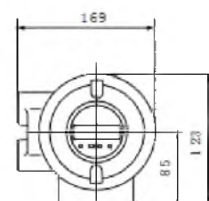
e Outline Dimension of medium and high pressure sensor M A G Y N Intelligence Transmitter (Round Type)
