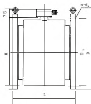
c Separate Type (≥DN 100)
